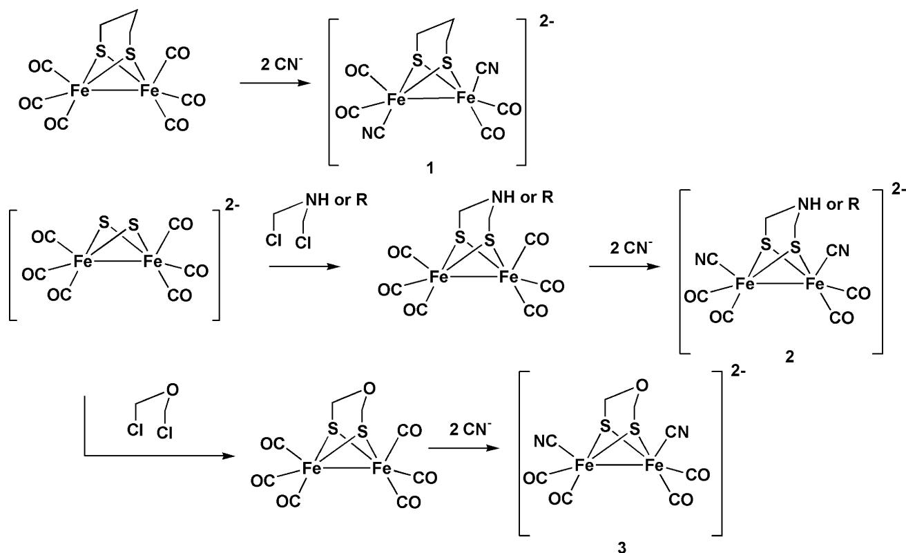
Scheme 2. Synthesis of \{2\text{Fe}2\text{S}_2\} -subsite analogues.
