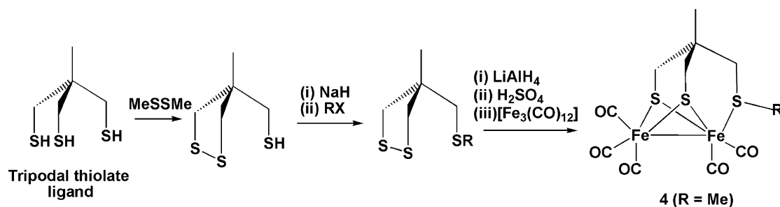
Scheme 3. Synthesis of \{2\text{Fe}_3\text{S}\} -complexes. The synthetic pathway offers considerable scope for varying the functionality R.
