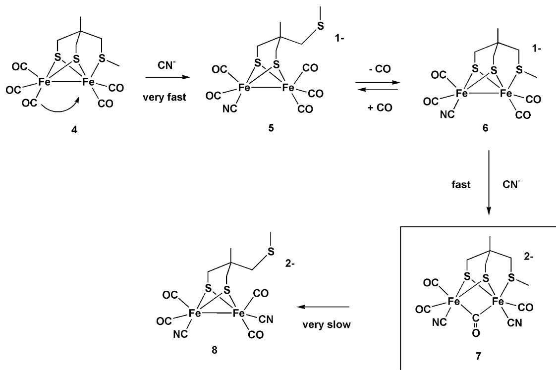
Scheme 4. The cyanide substitution pathway of \{2\text{Fe}_3\text{S}\} -subsite as deduced from stopped-flow FTIR kinetic analysis and labelling studies.
