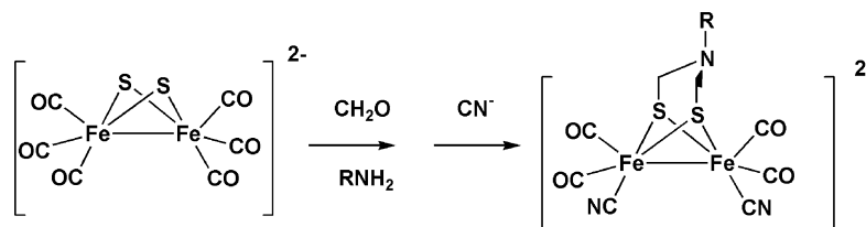
Scheme 5. ‘One-pot’ syntheses of azathiolate complexes.
