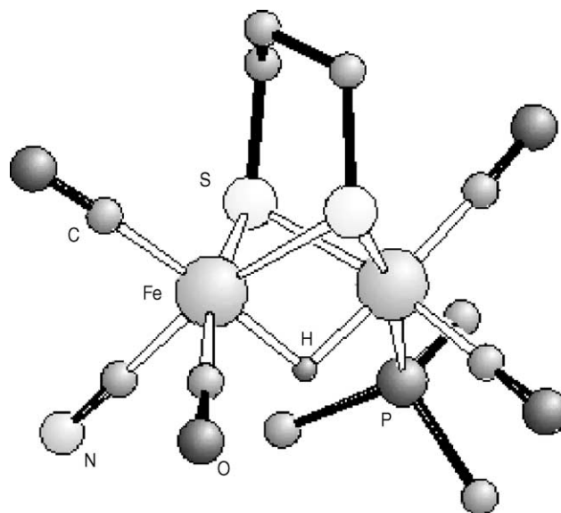
Fig. 6. X-ray structure of \mathbf{12} showing the hydride ligand bridging the two iron atoms.
