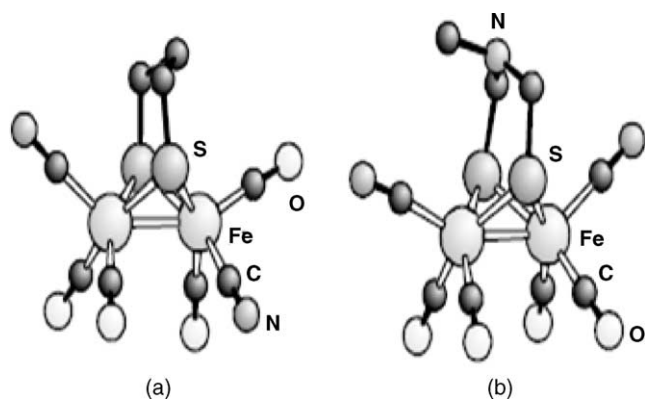
Fig. 2. Analogues of the subsite of the H-cluster possessing a 2\text{Fe}2\text{S}_2 -framework and CO/CN ligation. The analogues have structural features of CO inhibited form of the enzyme. Notice the different positional geometry of CN and CO ligands in complex (a) compared with (b). Reprinted with permission of the Royal Society of Chemistry (ref. [5]).
